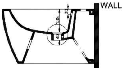
SECTION_VIEW A-A
