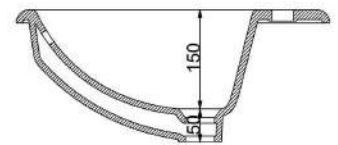
SECTION_VIEW A-A
