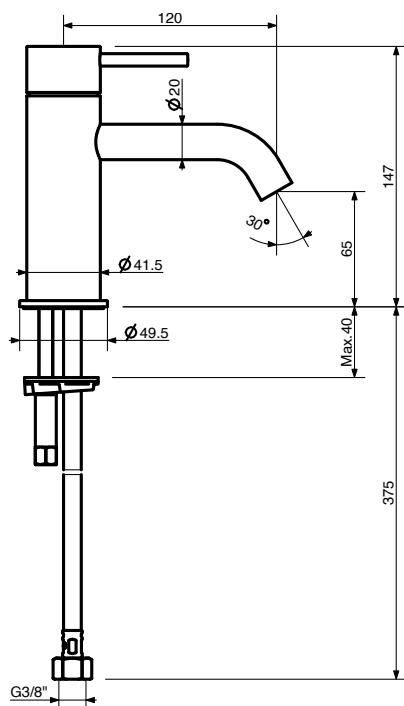
Art. XTR301
