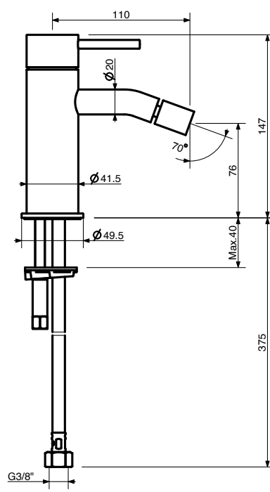
Art. XTR400
