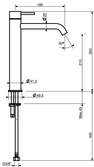
Art. XTR303
