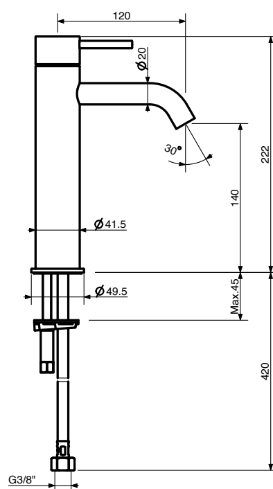
Art. XTR302
