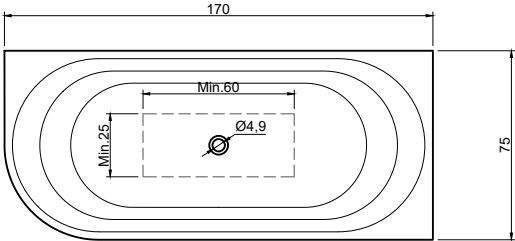
(Vasca decentrata sx o dx - versione SX / Off-center bathtub LH or RH - left version) art. OASI50S peso lordo/gross weight: kg 138 ca peso netto/net weight: kg 113 ca
