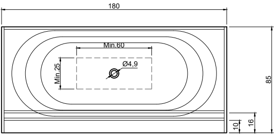
(Vasca centrale / Centered bathtub) art. OASI84MC peso lordo/gross weight: kg 149 ca peso netto/net weight: kg 124 ca
