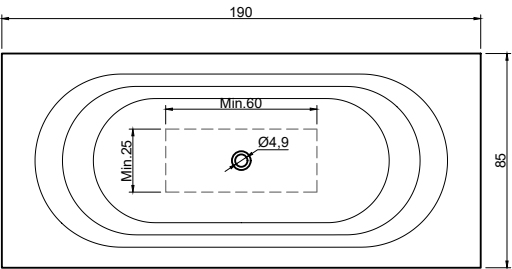
(Vasca centrale / Centered bathtub)
