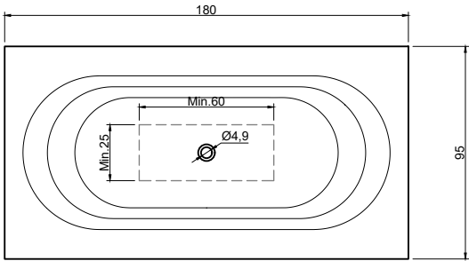
(Vasca centrale / Centered bathtub)
