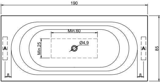
(Vasca centrale / Centered bathtub) art. OASI75MC peso lordo/gross weight: kg 153 ca peso netto/net weight: kg 128 ca
