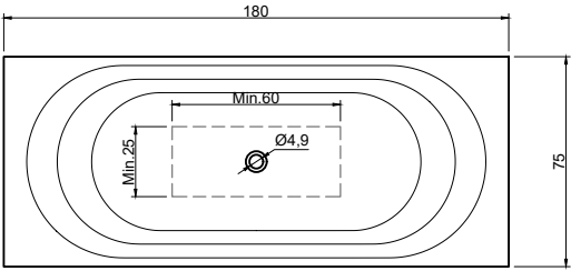
(Vasca centrale / Centered bathtub) art. OASI31C peso lordo/gross weight: kg 87 ca peso netto/net weight: kg 62 ca
