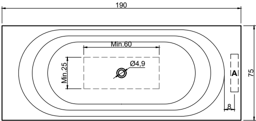
(Vasca centrale / Centered bathtub) art. OASI72C peso lordo/gross weight: kg 146 ca peso netto/net weight: kg 121 ca
