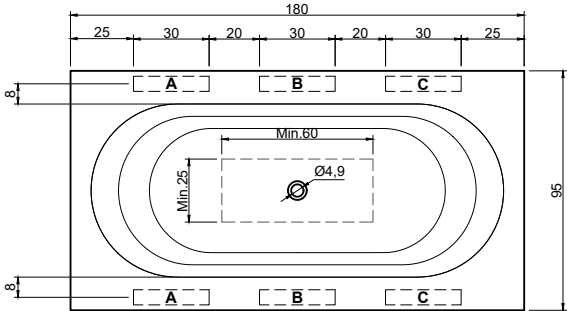
(Vasca centrale / Centered bathtub) art. OASI77MC peso lordo/gross weight: kg 156 ca peso netto/net weight: kg 131 ca
