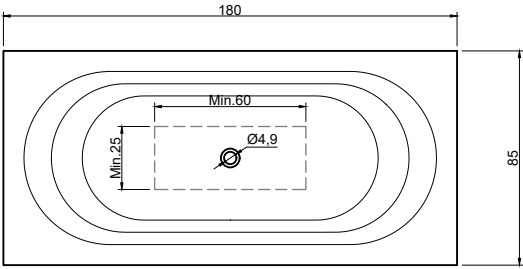
(Vasca centrale / Centered bathtub) art. OASI74MC peso lordo/gross weight: kg 149 ca peso netto/net weight: kg 124 ca
