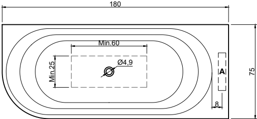
(Vasca decentrata sx o dx - versione SX / Off-center bathtub LH or RH - left version) art. OASI51S peso lordo/gross weight: kg 142 ca peso netto/net weight: kg 117 ca
