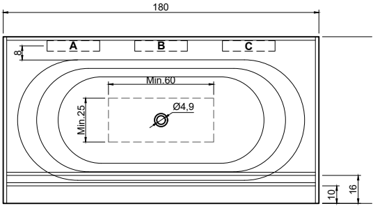
(Vasca centrale / Centered bathtub) art. OASI87MC peso lordo/gross weight: kg 149 ca peso netto/net weight: kg 124 ca
