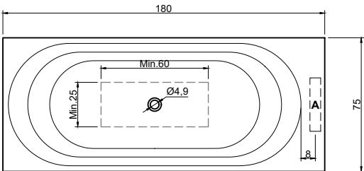
(Vasca decentrata sx o dx - versione SX / Off-center bathtub LH or RH - left version) art. OASI71S peso lordo/gross weight: kg 142 ca peso netto/net weight: kg 117 ca
