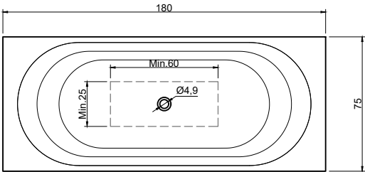
(Vasca centrale / Centered bathtub) art. OASI71C peso lordo/gross weight: kg 142 ca peso netto/net weight: kg 117 ca
