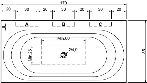
(Vasca decentrata in basso / Off-center bathtub in depth) art. OASI73F peso lordo/gross weight: kg 144 ca peso netto/net weight: kg 119 ca
