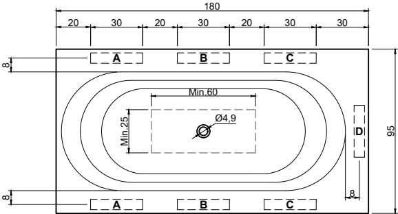
(Vasca decentrata sx o dx - versione SX / Off-center bathtub LH or RH - left version) art. OASI77MS peso lordo/gross weight: kg 156 ca peso netto/net weight: kg 131 ca
