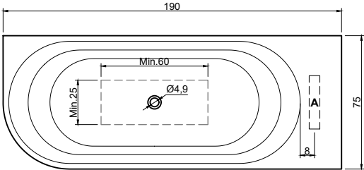
(Vasca decentrata sx o dx - versione SX / Off-center bathtub LH or RH - left version) art. OASI52S peso lordo/gross weight: kg 146 ca peso netto/net weight: kg 121 ca
