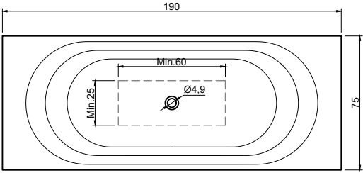
(Vasca centrale / Centered bathtub) art. OASI32C peso lordo/gross weight: kg 89 ca peso netto/net weight: kg 64 ca
