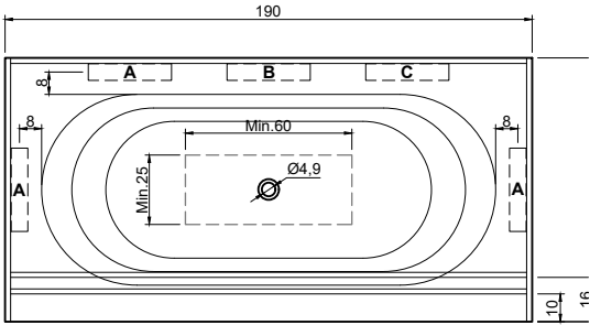
(Vasca centrale / Centered bathtub) art. OASI88MC peso lordo/gross weight: kg 153 ca peso netto/net weight: kg 128 ca
