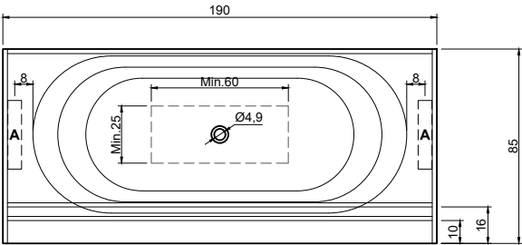
(Vasca centrale / Centered bathtub) art. OASI85MC peso lordo/gross weight: kg 153 ca peso netto/net weight: kg 128 ca
