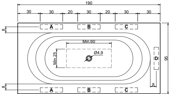
(Vasca centrale / Centered bathtub) art. OASI78MC peso lordo/gross weight: kg 159 ca peso netto/net weight: kg 134 ca
